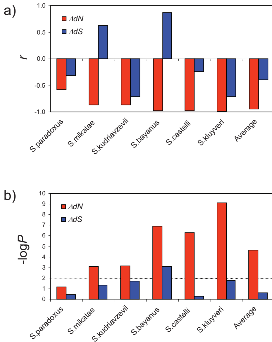
Figure 2. a) Pearson correlation ( r ) values are shown for the plots of distance difference ( \Delta dN & \Delta dS ) vs. GO functional similarity (sGO) in Figure 1. b) Statistical significance ( -\log P ) values are shown for the correlations in panel a. The P < 0.01 confidence level ( -\log P = 2 ) is shown. \Delta dN related values are shown in red and \Delta dS related values are shown in blue. Species are ordered left-to-right in terms of increasing evolutionary distance from S. cerevisiae .
