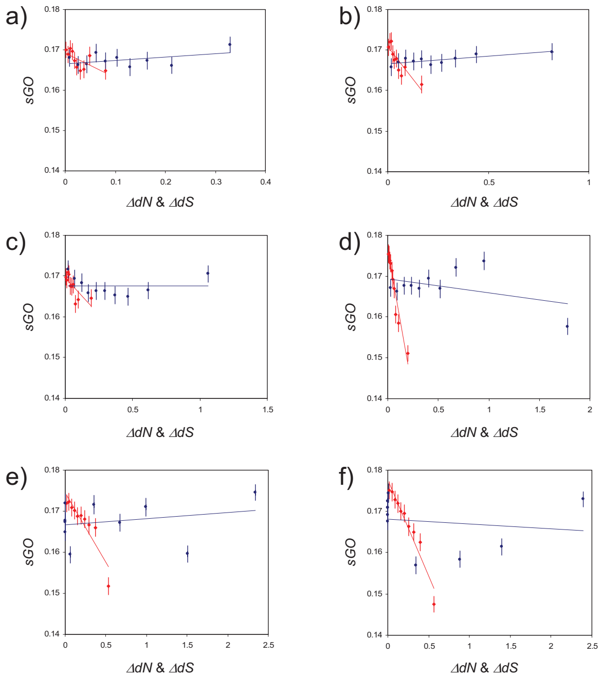
Figure 1. Average pairwise distance differences (x-axis) for 10 bins, with \Delta dN shown in red and \Delta dS shown in blue, are plotted against average pairwise GO functional similarities ( sGO on the y-axis). The error bars correspond to 99% confidence intervals. Distances were calculated between orthologous genes of S. cerevisiae and a) S. paradoxus , b) S. mikatae , c) S. kudriavzevii , d) S. bayanus , e) S. castellii , f) S. kluyveri .
