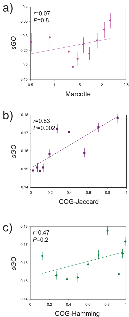
Figure 3. Phylogenetic profile similarity (x-axis) versus GO functional similarity (sGO on the y-axis). sGO is compared to a) Marcotte profiles, b) COG profiles evaluated via Jaccard similarity and c) COG profiles evaluated via Hamming similarity. Pearson correlation ( r ) and significance ( P ) values are shown in the inset of each plot.
